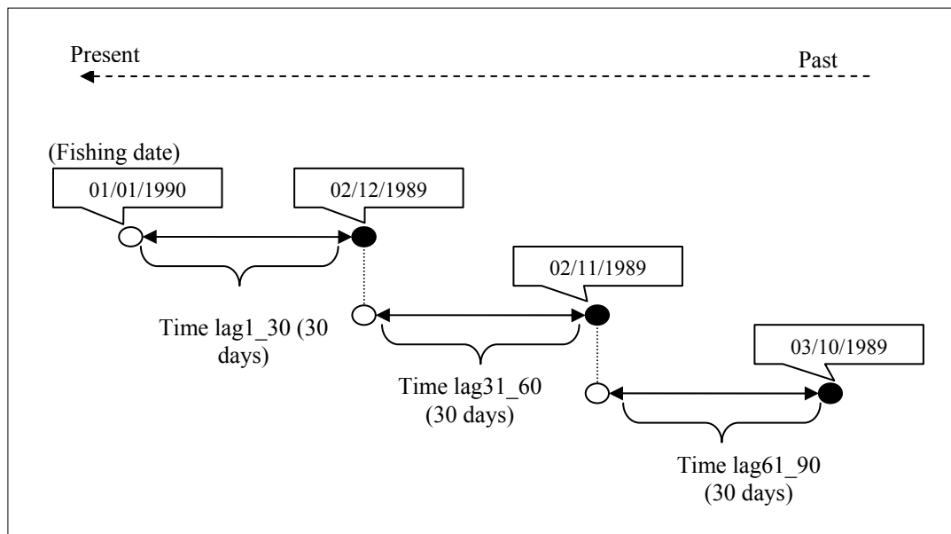
Figure 3.3 Illustration showing how the time-lagged rainfall and river flow measurements were calculated for a banana prawn catch reported on 01/01/1990. Closed circles include a date noted in the diagram, and open circles do not include dates in the diagram.
