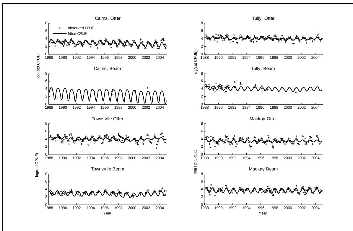
Figure 5.6 Observed (circles) and predicted (lines) standardised (log-scaled) CPUE from age-structured base model (Model D) in northern region (Cairns to Mackay).
