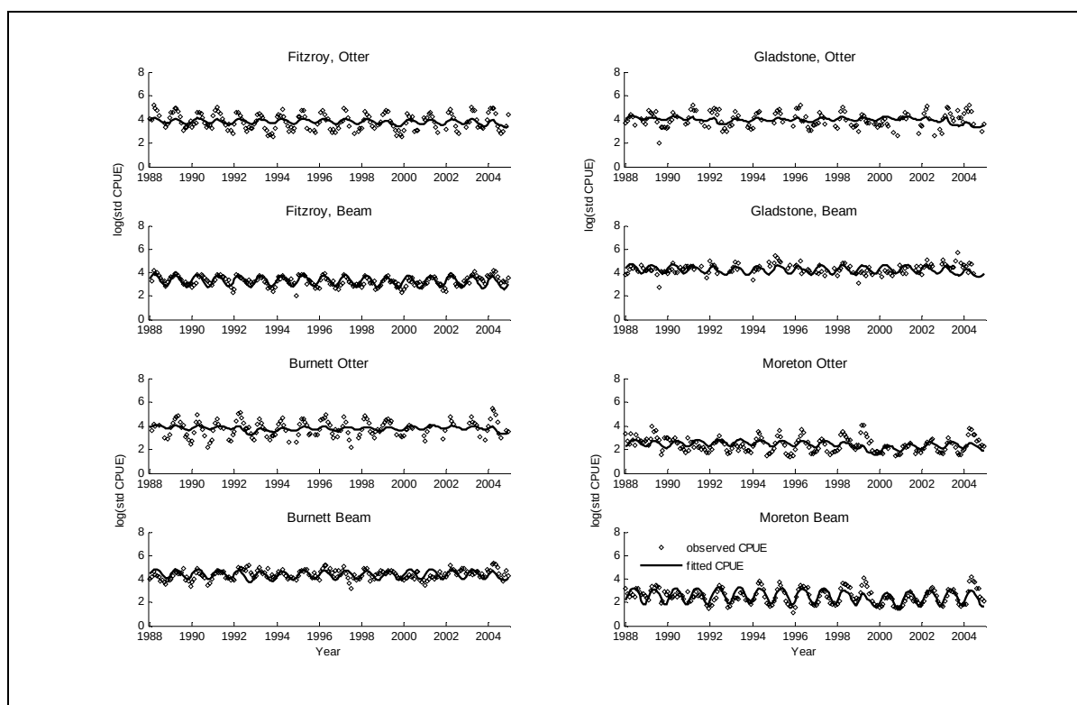
Figure 5.7 Observed (circles) and predicted (lines) standardised (log-scaled) CPUE from age-structured base model (Model D) in southern region (Fitzroy to Moreton).
