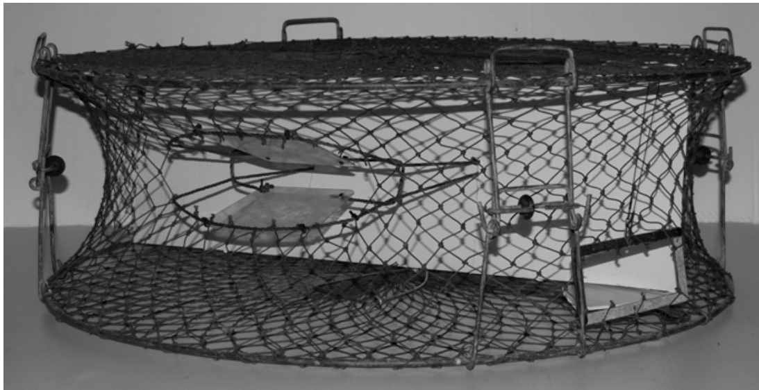
Figure 7.1. A polyethylene-mesh pot with escape vent (bottom right) fitted perpendicular to funnel (left of centre). A white plastic panel obscures the rear of the pot and was inserted to highlight design features only.
