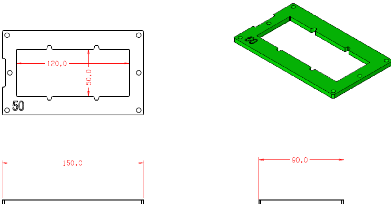
Figure 22.2. Schematics for 120 mm x 50 mm (W x H) escape vents (sized to retain Scylla serrata \geq 150 mm carapace width) produced by Lincoln Plastics. Device thickness is 5 mm. The holes in the middle of the short edges have since been removed as they caused weak points. Likewise, the recess on the left side of the device has also been removed.
