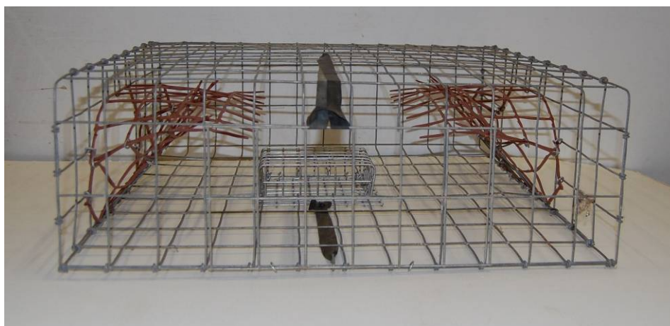
Figure 2.3. A wire-mesh pot with two funnels and central bait box. The upper and lower rubber straps hold closed the doors to the main chamber and bait box, respectively.
