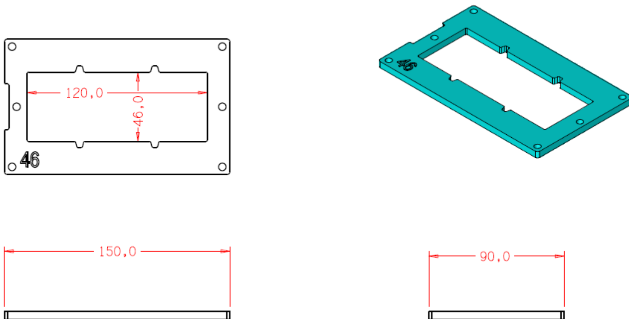
Figure 22.1. Schematics for 120 mm x 46 mm (W x H) escape vents (sized to retain Scylla serrata \geq 140 mm carapace width) produced by Lincoln Plastics. Device thickness is 5 mm. The holes in the middle of the short edges have since been removed as they caused weak points. Likewise, the recess on the left side of the device has also been removed.
