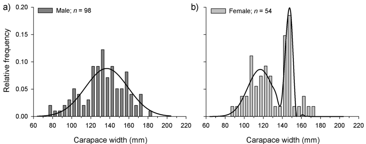
Figure 7.5 Relative size frequency of unique a) male and b) female Scylla serrata caught in polyethylene-mesh pots set in the Roper River. Upper bin values for each 5-mm size category end with 4 or 9. Parameter values and correlation coefficients for Gaussian curves are given in Appendix 3.
