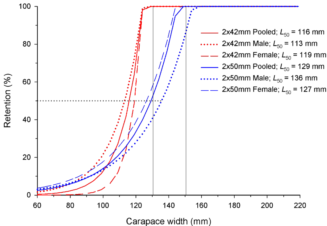
Figure 7.7. Pooled and sex-specific selectivity curves (Richards' functions with estimated p ) for Scylla serrata caught in 2x42mm (red lines) and 2x50mm (blue lines) vented polyethylene-mesh pots set in the Adelaide River. The horizontal dotted line intersects the length at 50% retention ( L_{50} ) for each curve. The left and right vertical lines represent the minimum legal sizes for males harvested by the NT recreational fishery and the Qld mud crab fishery, respectively.
