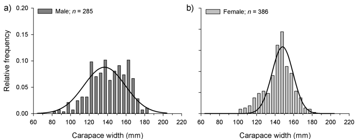
Figure 6.4. Relative size frequency of unique male a) and female b) Scylla serrata caught in wire-mesh pots set in the Roper River. Upper bin values for each 5-mm size category end with 4 or 9. Parameter values and correlations coefficients for Gaussian curves are given in Appendix 3.
