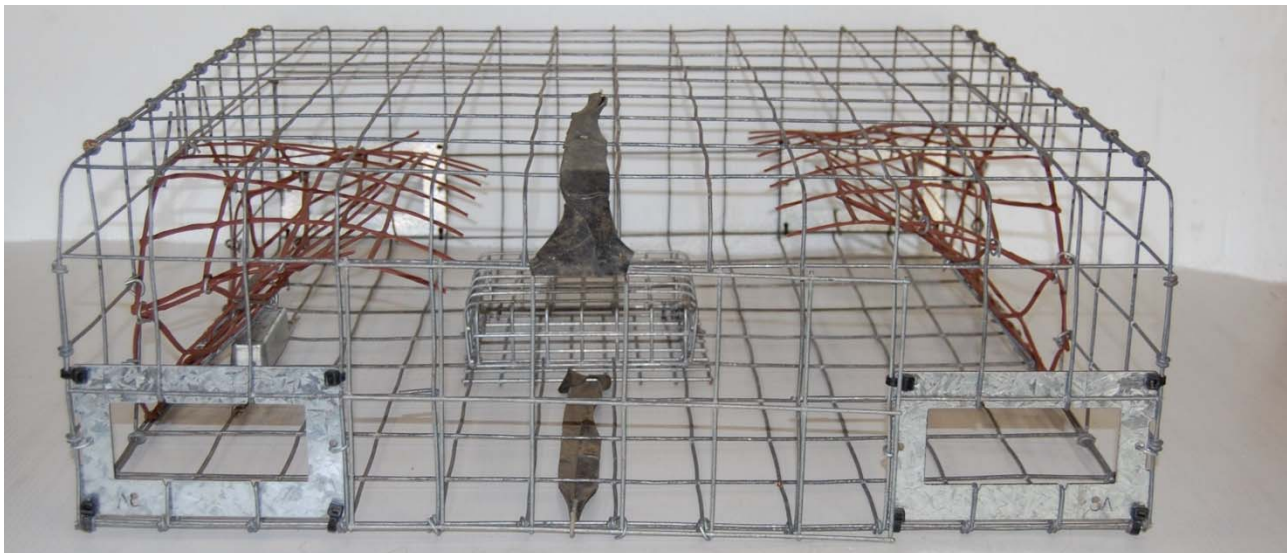
Figure 6.1. A wire-mesh pot with four escape vents fitted
