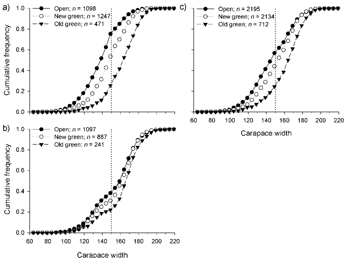
Figure 8.12. Cumulative size frequency of Scylla serrata caught in polyethylene-mesh pots in areas of the Moreton Bay Marine Park open to fishing (Open), closed to fishing since 1 March 2009 (New green) and closed to fishing since 1 December 1997 (Old green). Plots a) and b) show data for males and females, respectively. Plot c) shows data for both sexes combined. Upper bin values for each 5-mm size category end with 4 or 9. The dotted vertical line shows the minimum legal size for males harvested by the Qld mud crab fishery.
