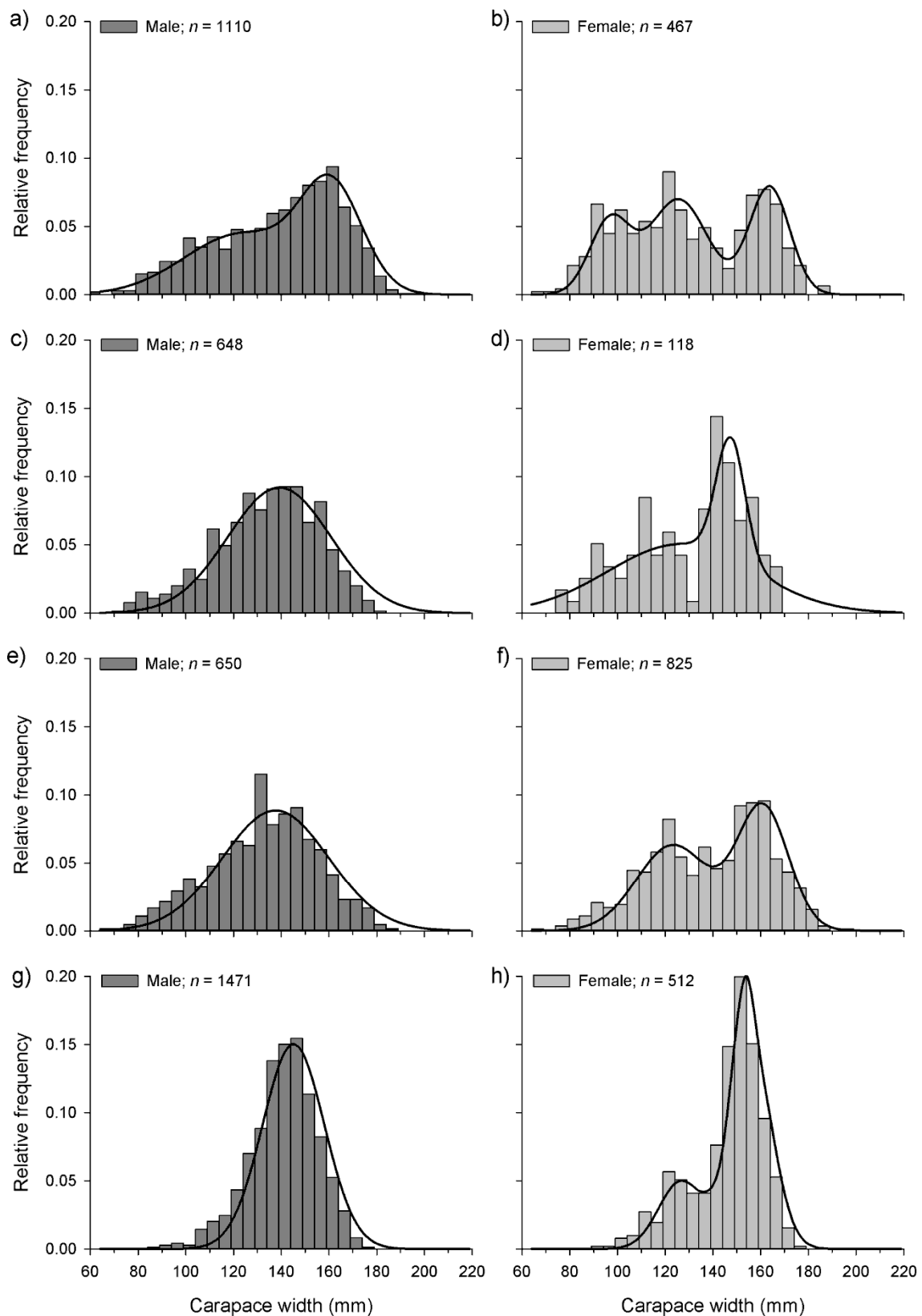
Figure 8.6. Relative size frequency of male (left) and female (right) Scylla serrata caught in polyethylene-mesh pots set in the Gulf of Carpentaria (a,b), the far north (c,d), the northern wet (e,f) and the northern dry (g,h) regions of Qld. Upper bin values for each 5-mm size category end with 4 or 9. Parameter values and correlation coefficients for Gaussian curves given in Appendix 3.
