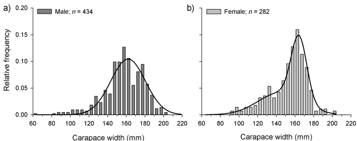
Figure 7.4 Relative size frequency of unique a) male and b) female Scylla serrata caught in polyethylene-mesh pots set in the Adelaide River. Upper bin values for each 5-mm size category end with 4 or 9. Parameter values and correlation coefficients for Gaussian curves given in Appendix 3.
