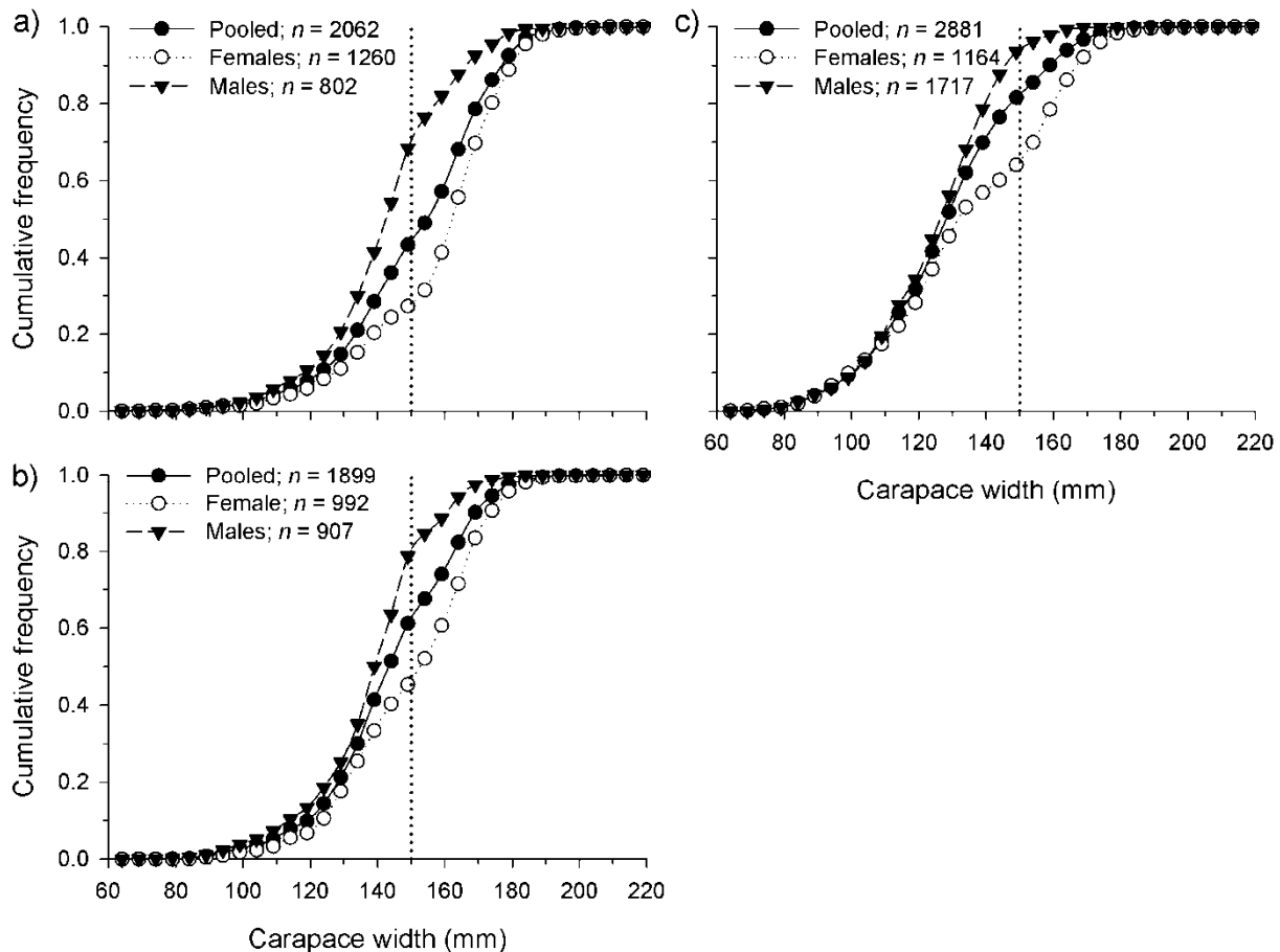
Figure 8.10. Pooled and sex-specific cumulative size frequency of Scylla serrata caught in polyethylene-mesh pots set in a) the Capricorn, b) the Fraser-Burnett and c) the Moreton Bay regions of Qld. Upper bin values for each 5-mm size category end with 4 or 9. The dotted vertical line shows the minimum legal size for males harvested by the Qld mud crab fishery.
