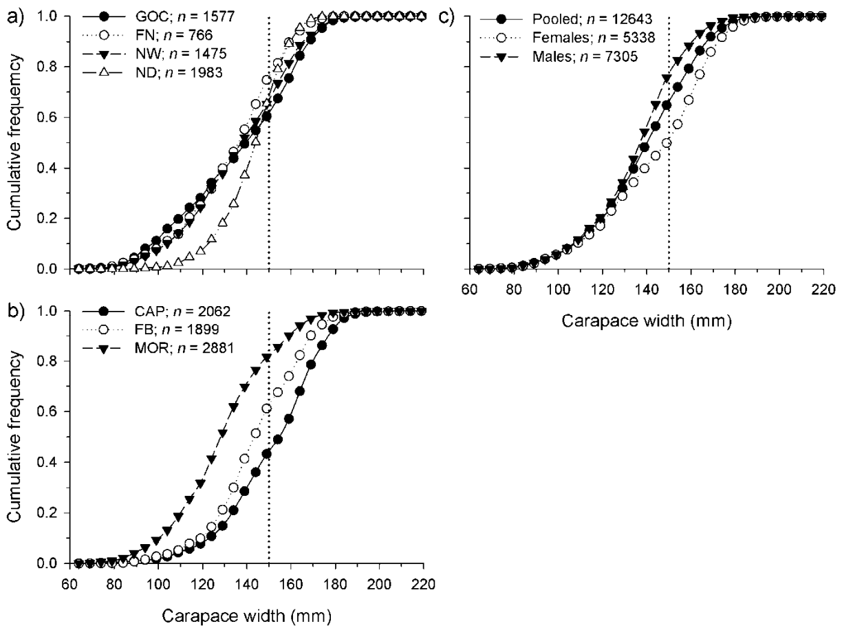
Figure 8.8 Cumulative size frequency of Scylla serrata caught in polyethylene-mesh pots set in the Gulf of Carpentaria (GOC), far north (FN), northern wet (NW), northern dry (ND), Capricorn (CAP), Fraser-Burnett (FB) and Moreton Bay (MOR) regions of Qld. Plots a) and b) show data (pooled across sex) for northern and southern regions, respectively. Plot c) shows pooled and sex specific data for all areas combined. Upper bin values for each 5-mm size category end with 4 or 9. The dotted vertical line shows the minimum legal size for males harvested by the Qld mud crab fishery.
