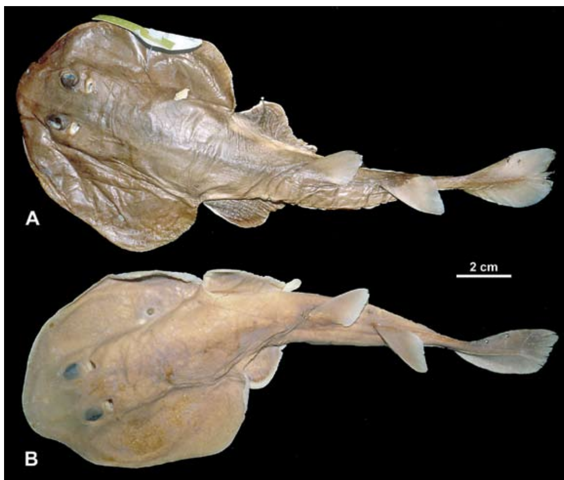
Figure 13. Dorsal views of (A) Narcine tasmaniensis Richardson, 1841 (CSIRO H 949–12, 360 mm TL adult male) and (B) Narcine lasti Carvalho and Séret, 2002 (CSIRO H 2597–09, 302 mm TL adult male), from off Sydney, off New South Wales and Western Australia, respectively.
