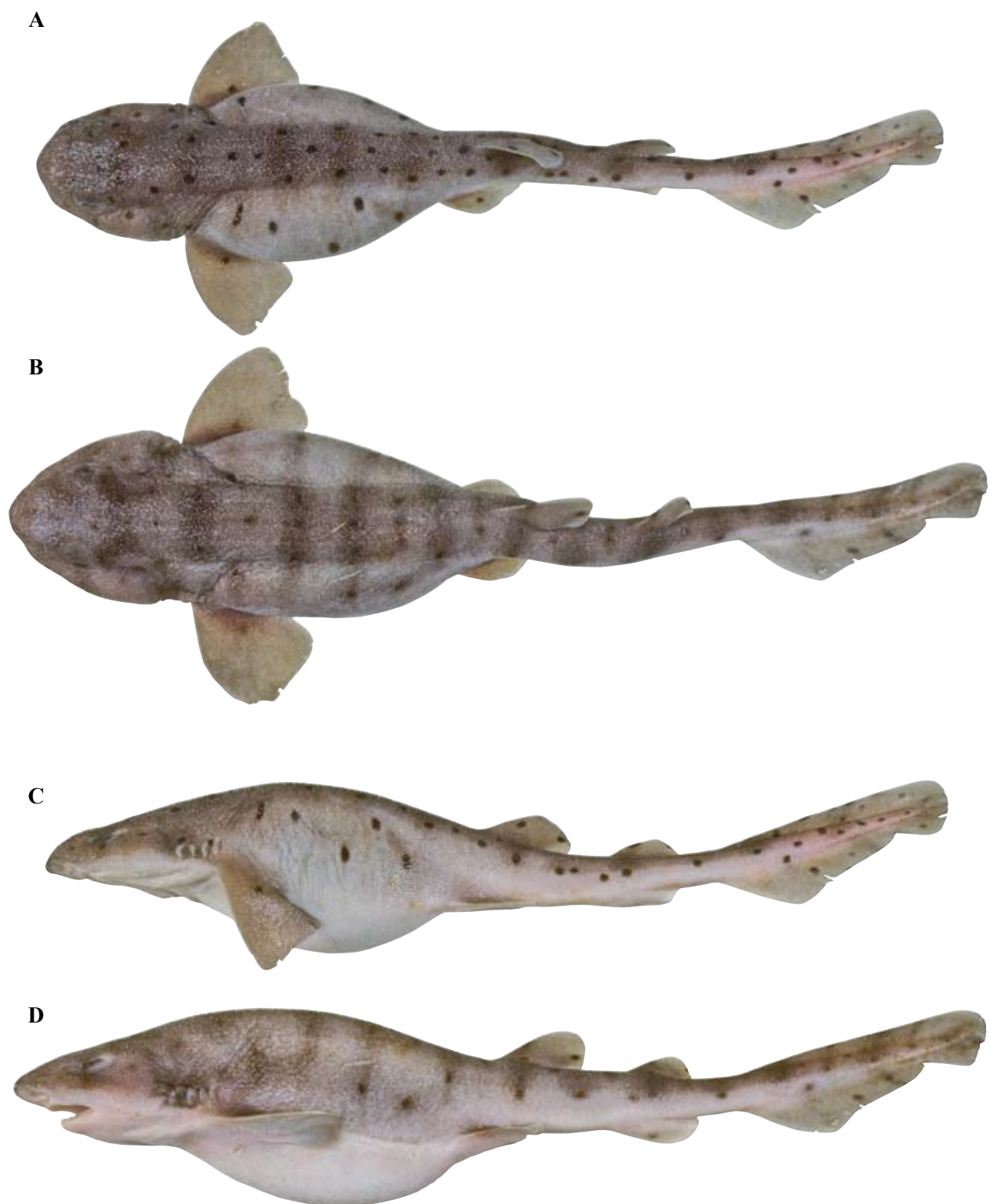
Figure 2. Cephaloscyllium variegatum sp. nov.: A. dorsal view of paratype CSIRO H 4684-01 (female 237 mm TL); B. dorsal view of paratype CSIRO H 4684-02 (juvenile male 252 mm TL); C. lateral view of paratype CSIRO H 4684-01 (female 237 mm TL); D. lateral view of paratype CSIRO H 4684-02 (juvenile male 252 mm TL).
