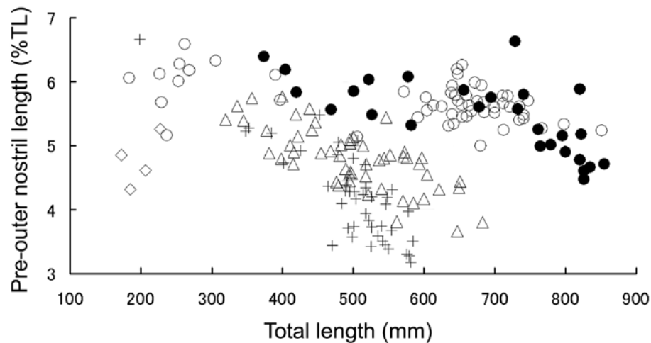
Figure 12. Ratio of pre-outer nostril length in Apristurus ampliceps sp. nov. (●), A. fedorovi (Δ), A. kampae (+), A. manis (○) and A. stenseni (◇).
