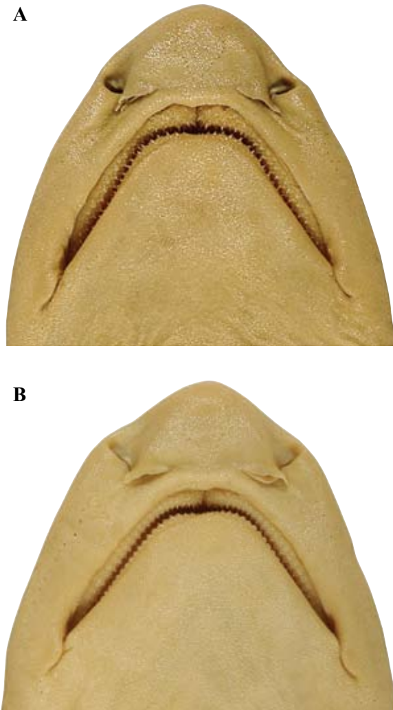
Figure 8. Ventral view of head of Cephaloscyllium zebrum sp. nov.: A. holotype CSIRO H 1323-02 (adult male 445 mm TL); B. paratype CSIRO H 1323-03 (female 435 mm TL).
