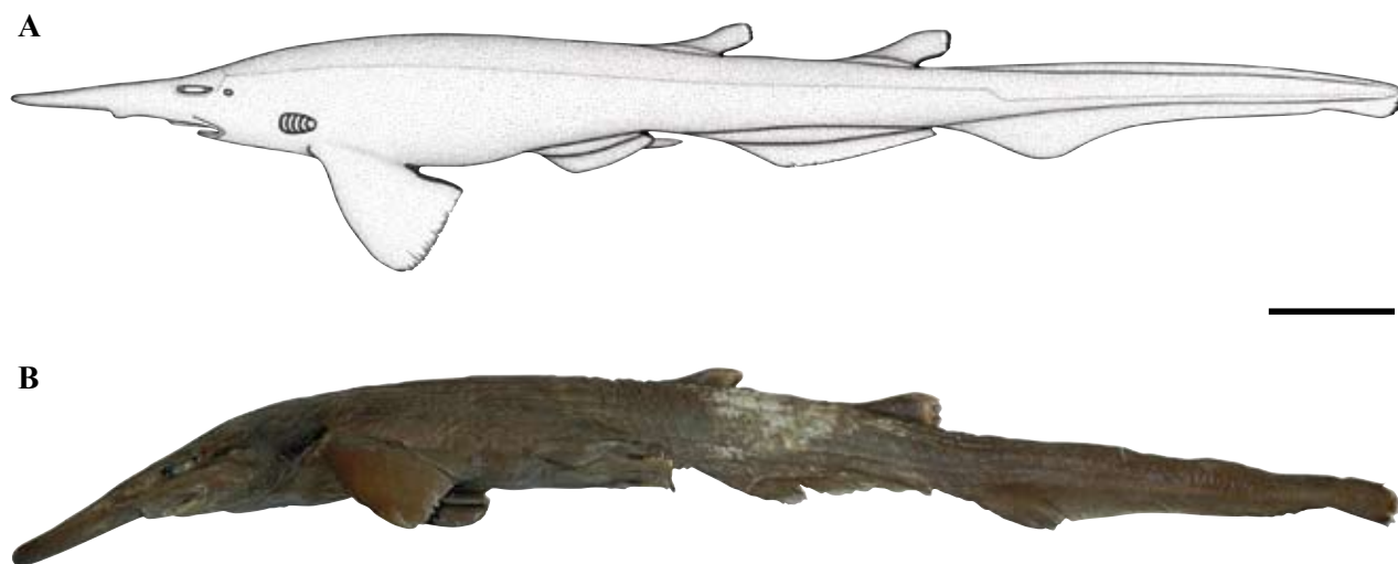
Figure 1. Apristurus australis sp. nov., holotype CSIRO H 953–07 (mature male 616 mm TL): A. lateral view (drawing); B. lateral view (photograph). Scale bar = 50 mm.
