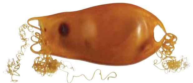
Figure 4. Egg case of Cephaloscyllium variegatum sp. nov. (CSIRO B 2253).
