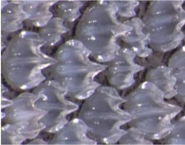
Figure 4. Cusps of the flank denticles of Glyphis garricki sp. nov., paratype WAM P 32598–001 (juvenile male 906 mm TL).
