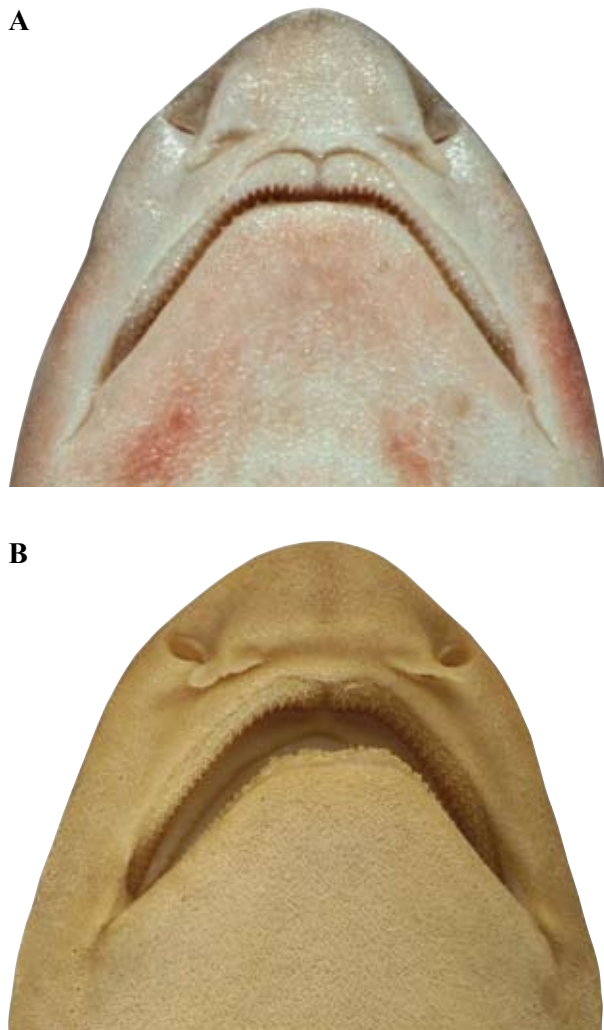
Figure 2. Ventral view of head of Cephaloscyllium hiscosellum sp. nov.: A. adult male holotype (CSIRO H 2590-07, 458 mm TL); B. female paratype (CSIRO CA 4484, female 336 mm TL).
