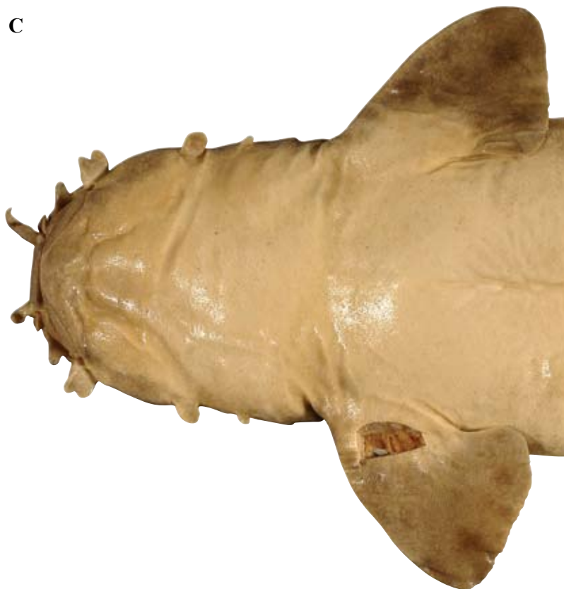
Figure 1. Orectolobus reticulatus sp. nov., adolescent male holotype (NTM S 13251–001, 503 mm TL, preserved): A. lateral view; B. dorsal view; C. ventral head and pectoral fins.
