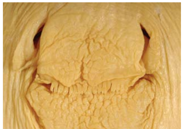
Figure 3. Oronasal region of Trygonoptera galba sp. nov., adult male holotype (NMV A 1793, 328 mm TL, preserved).
