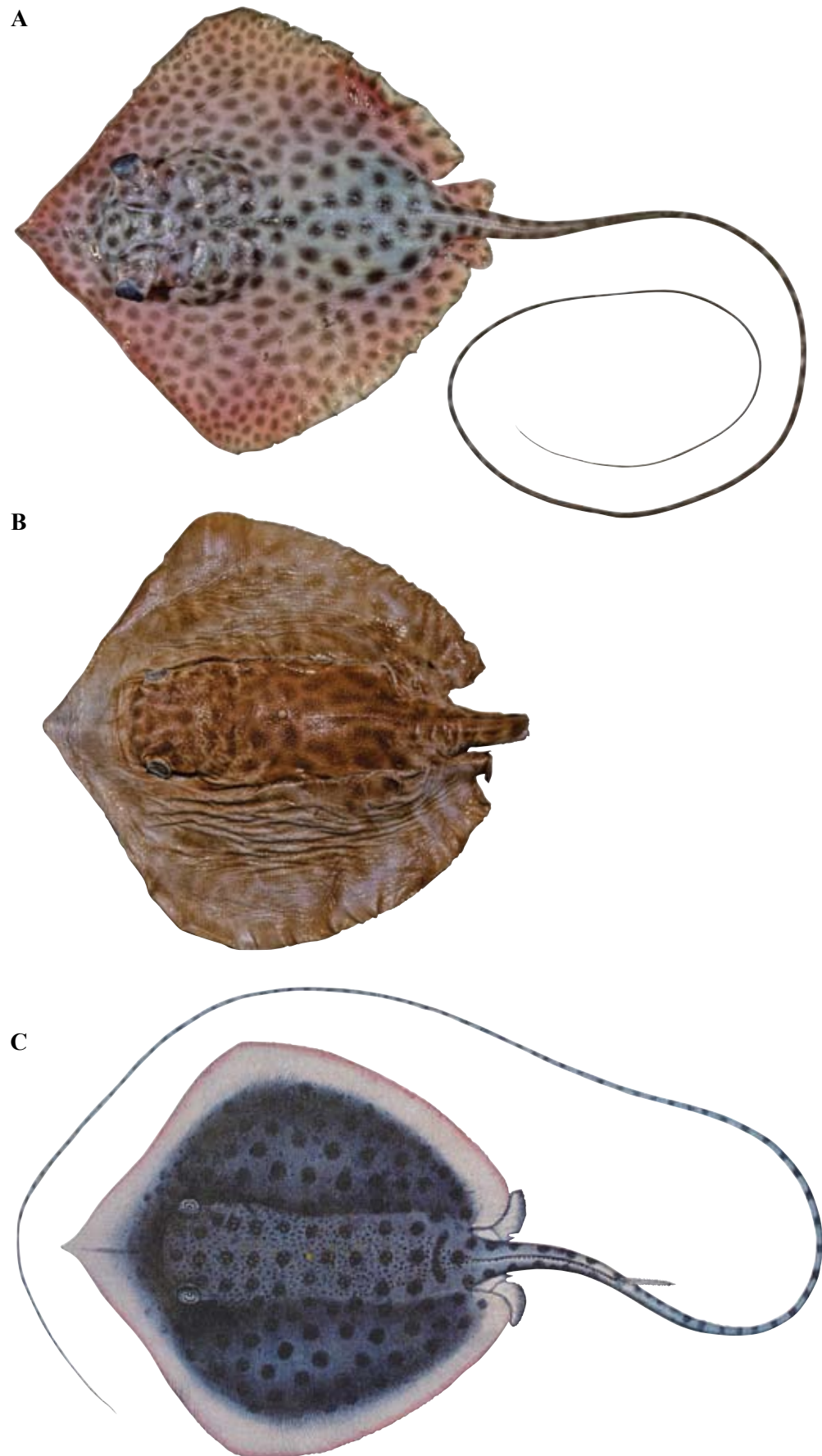
Figure 5. Dorsal view of: A. Himantura leoparda sp. nov., early juvenile paratype (CSIRO H 635–02, female 200 mm DW, preserved); B. Trygon undulata Bleeker, syntype (BMNH 1867.11.28.156, female 264 mm DW, preserved); C. Trygon russellii (original illustration by Gray).
