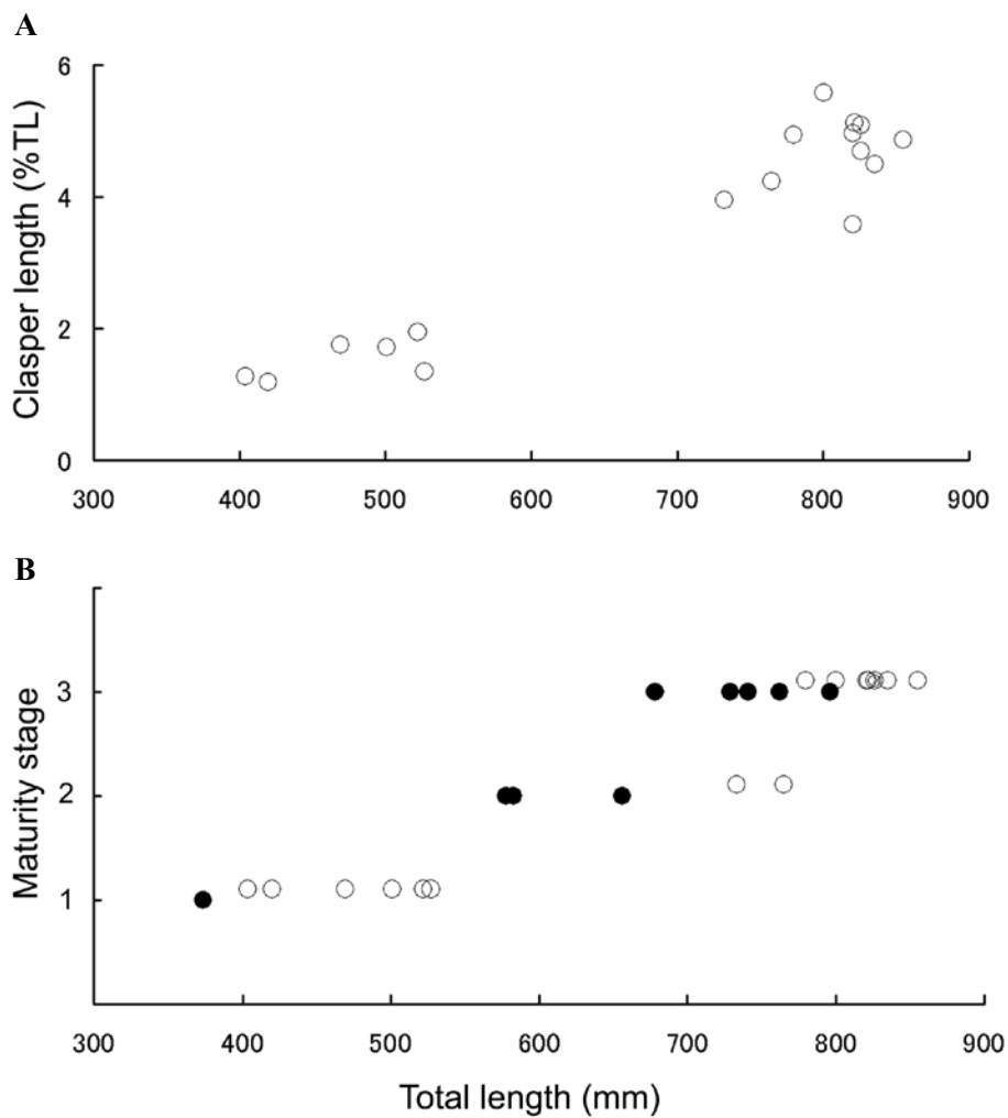
Figure 6. Clasper length (A) and sexual maturity stages (B) of Apristurus ampliceps sp. nov. Males (○) and females (●).
