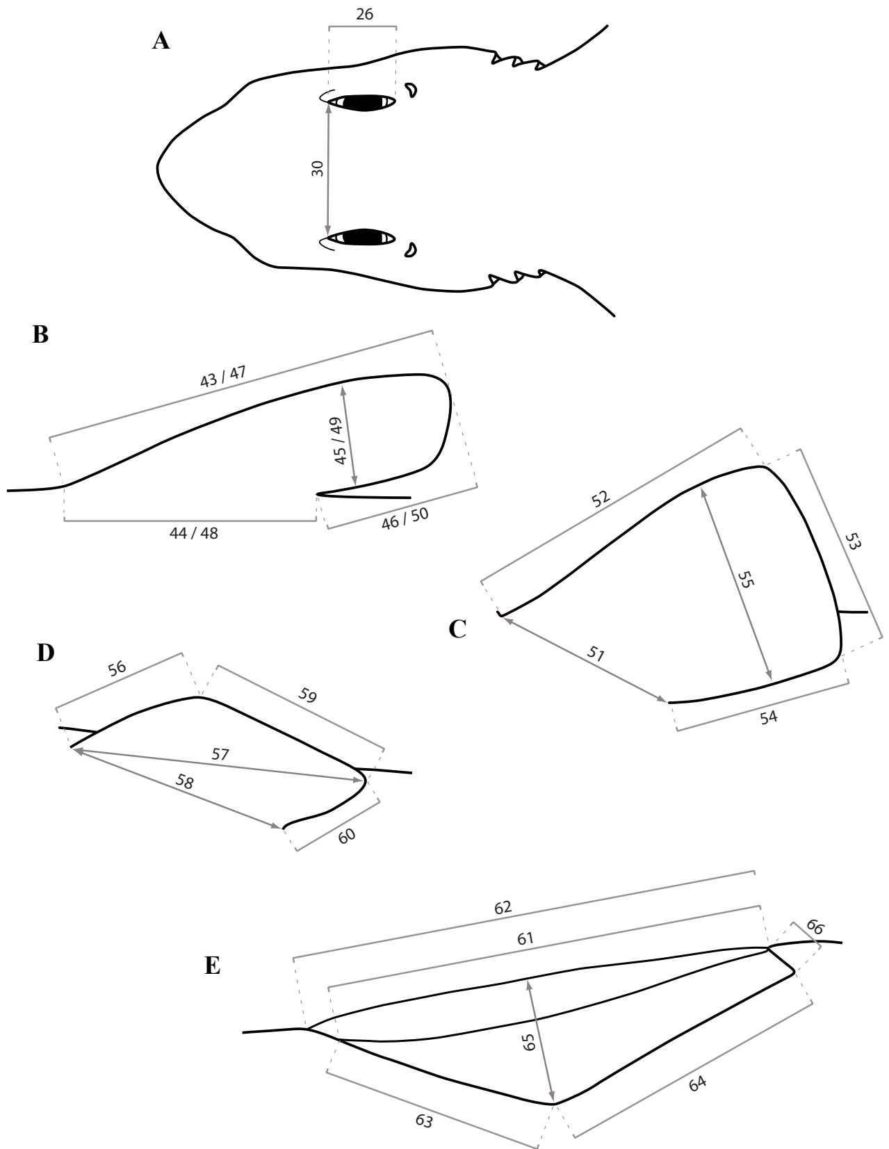
Figure 3. Dorsal view of head (A) and dorsal (B), pectoral (C), pelvic (D) and anal (E) fins of Apristurus , showing diagrammatic representation of the morphometric characters. Refer to Table 1 and text for definitions and explanation of measurements.
