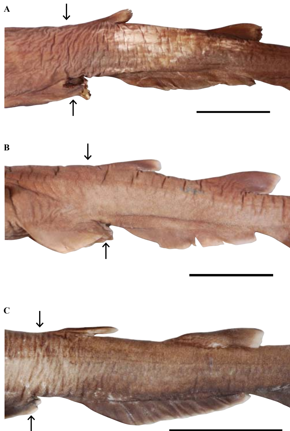
Figure 7. Positions of first dorsal-fin origin and pelvic-fin insertion (arrows): A. Apristurus australis sp. nov., holotype CSIRO H 953–07 (mature male 616 mm TL); B. Apristurus australis sp. nov., paratype CSIRO T 459 (mature female 562 mm TL); C. Apristurus herklotsi , HUMZ 170421 (mature female 482 mm TL). Scale bar = 50 mm.
