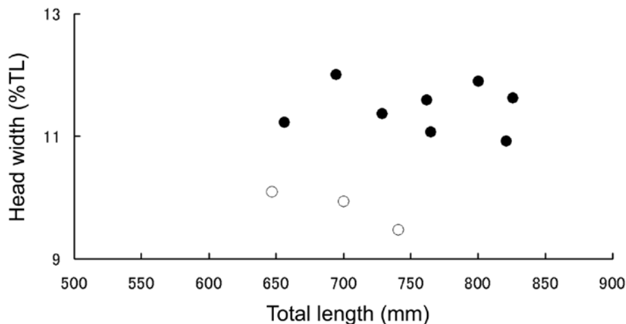
Figure 13. Ratio of head width in Apristurus ampliceps sp. nov. (●) and A. manis (○).
