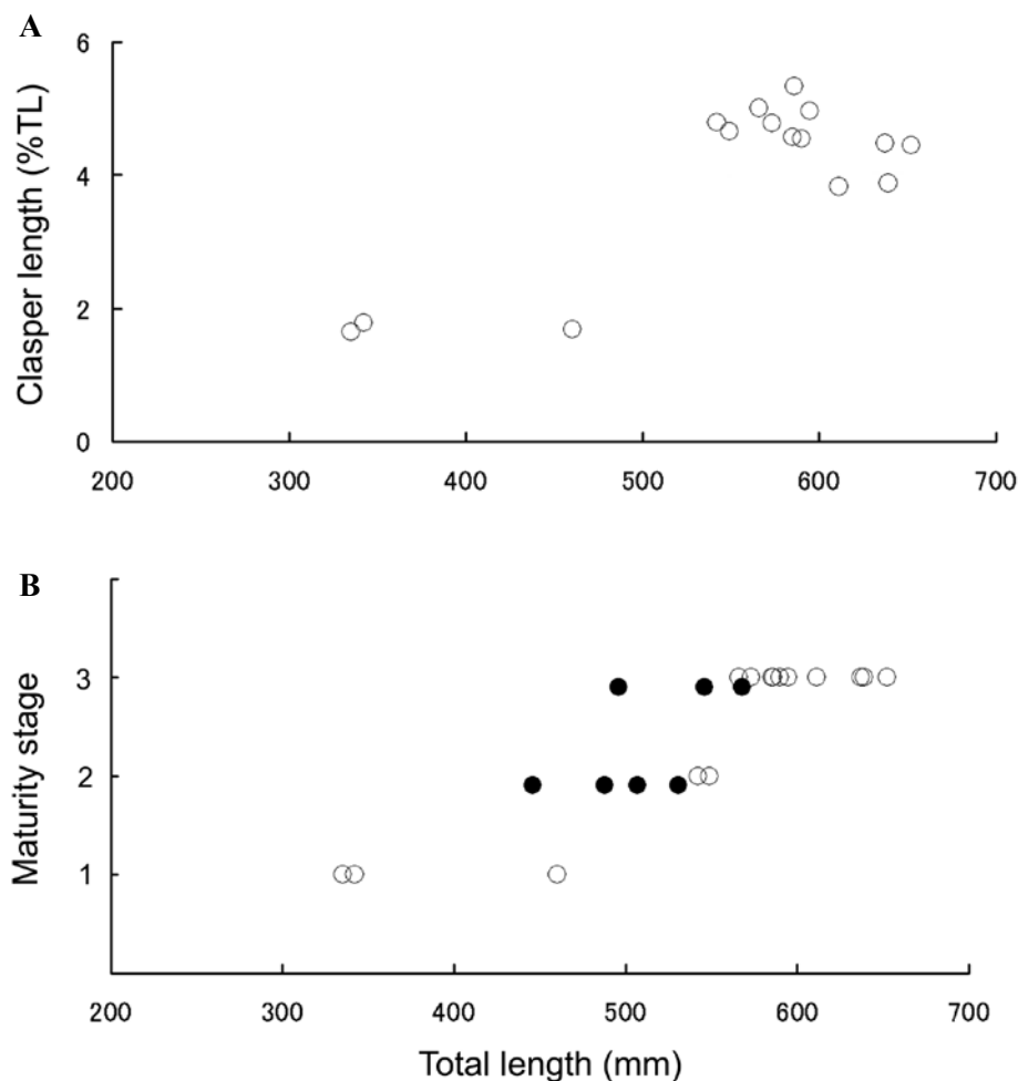
Figure 13. Clasper length (A) and sexual maturity stages (B) of A. pinguis from the Indian and the western South Pacific. Males (○), females (●).
