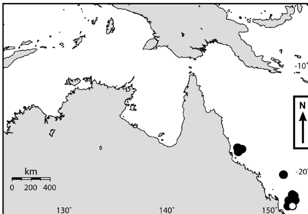
Figure 12. Map showing distribution of Narcine nelsoni sp. nov.; open circle is approximate locality of holotype.
