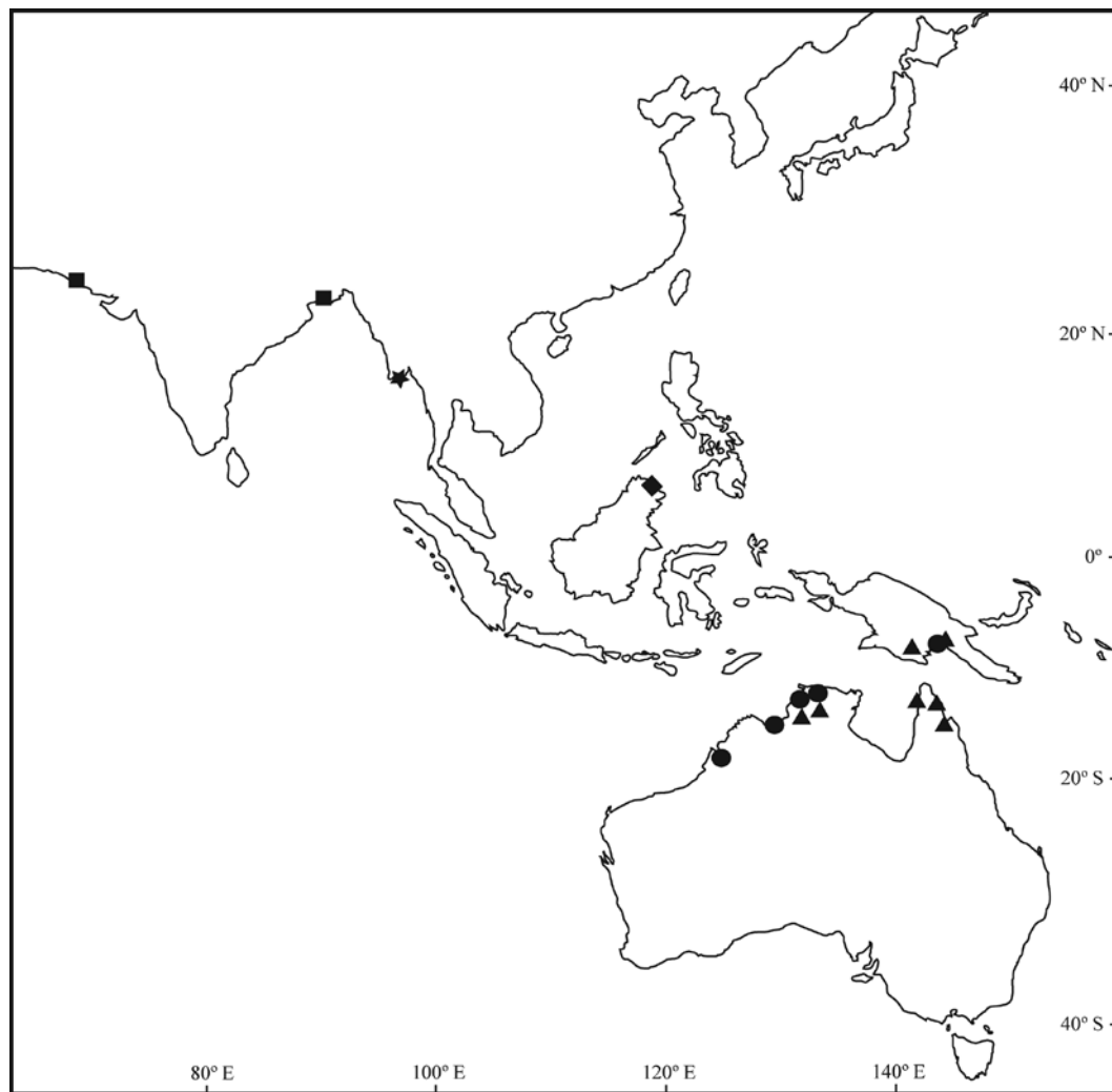
Figure 12. Map showing the collection localities of specimens of the known species of Glyphis : G. gangeticus (square), G. garricki (circle), G. glyphis (triangle), G. siamensis (star) and G. sp. B (diamond).
