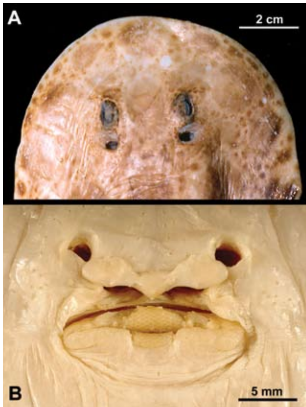
Figure 5. (A) Dorsal head region of paratype of Narcine ornata sp. nov. (QM I 27854, 237 mm TL adult female, Gulf of Carpentaria); (B) oronasal region of holotype of Narcine ornata sp. nov. (CSIRO H 3646-02, 186 mm TL adult male).
