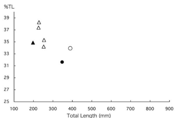
Figure 4. Scatter diagram of proportional dimensions of caudal length in the type specimens of Apristurus kampae and A. manis . Closed symbols, A. kampae ; open symbols, A. manis ; circles, holotypes; triangles, paratypes.
