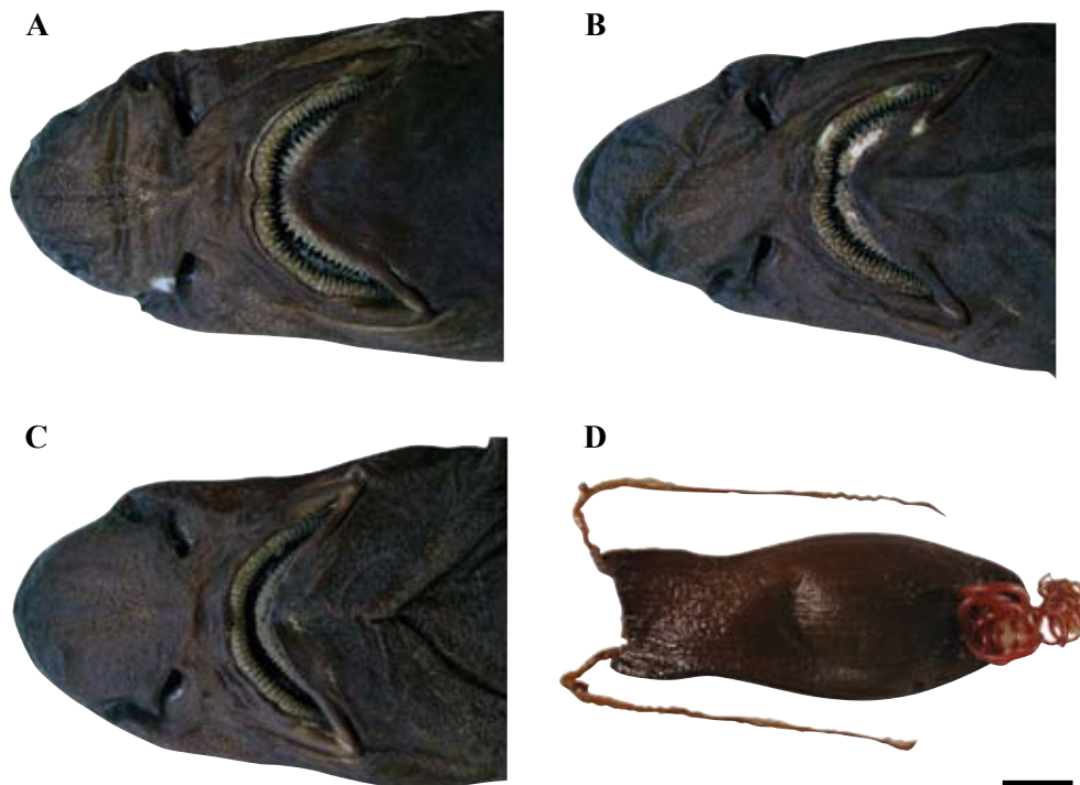
Figure 2. Ventral views of head (A–C) showing variation of snout shape and an egg capsule (D) of Apristurus melanoasper . A. Australian specimen, HUMZ 189942, male 684.5 mm TL; B. Australian specimen, HUMZ 139936, male 695.3 mm TL; C. North Atlantic specimen, MCZ 125408, paratype, male 692 mm TL; D. egg capsule from a New Zealand specimen, NMNZ P 16021, female 704 mm TL. Scale bar = 1 cm.
