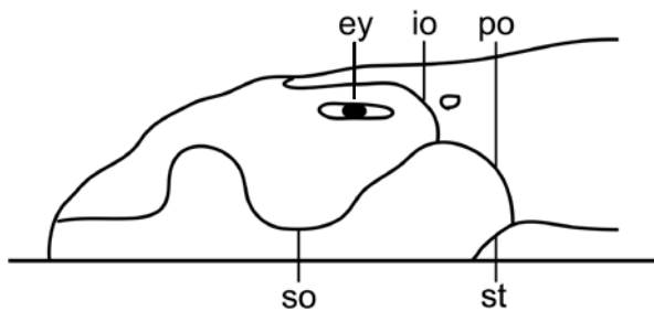
Figure 9. Sensory canal of head (right side) of Apristurus pinguis : HUMZ 139943, male 595 mm TL. Ey, eye; io, infraorbital canal; po, postorbital canal; so, supraorbital canal; st, supratemporal canal.
