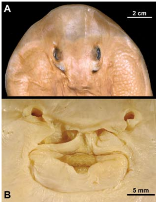
Figure 11. (A) Dorsal head region of paratype of Narcine nelsoni sp. nov. (QM I 22095, 257 mm TL adolescent or adult male, off Swain Reefs, Capricorn Channel, Queensland); (B) oronasal region of holotype of Narcine nelsoni sp. nov. (CSIRO H 719-06, 260 mm TL adult male).
