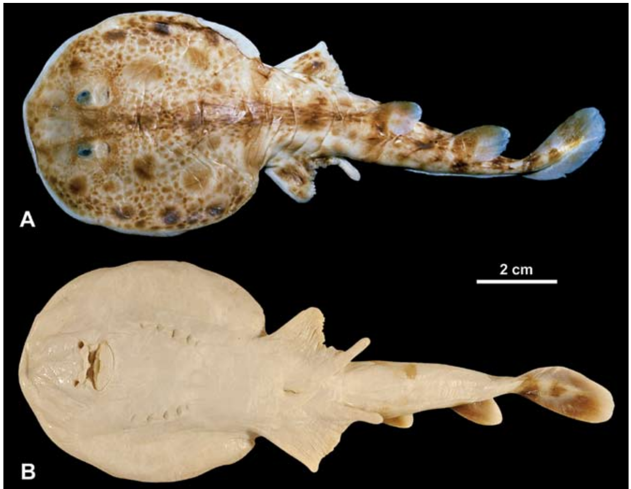
Figure 1. Holotype of Narcine ornata sp. nov. in dorsal (A) and ventral (B) views (CSIRO H 3646–02, 186 mm TL adult male, Gulf of Carpentaria, fresh). Caudal fin is downturned in ventral view.
