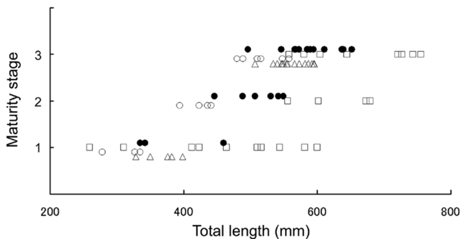
Figure 18. Sexual maturity stages: A. pinguis from the Indian and the western South Pacific (●) and from the East China Sea (○); A. albisoma (Δ) and A. profundorum (□).
