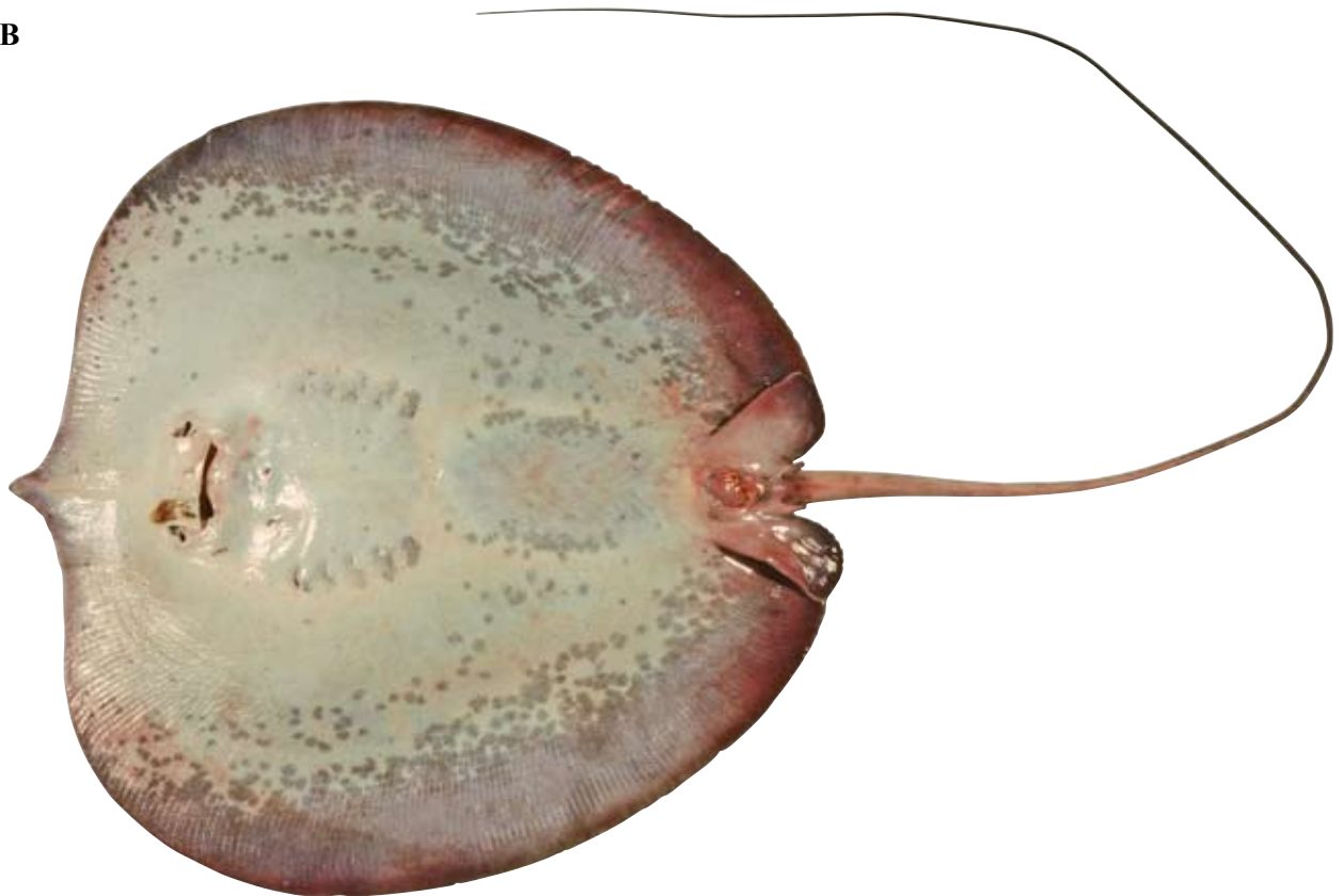
Figure 1. Himantura dalyensis sp. nov., juvenile male holotype (CSIRO H 2503–01, 620 mm DW, fresh): A. dorsal view; B. ventral view.
