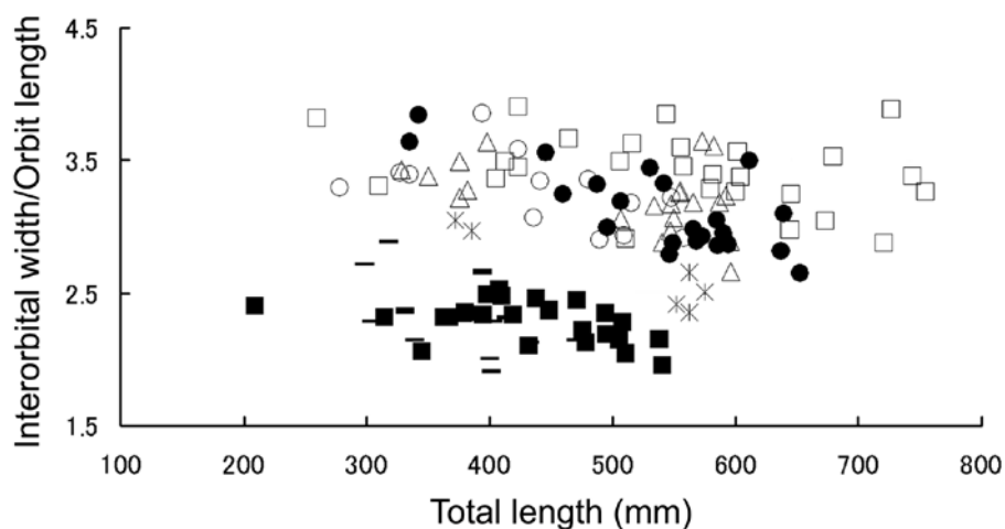
Figure 17. Ratio of orbit length in interorbital width: A. pinguis from the Indian and the western South Pacific (●) and from the East China Sea (○); A. albisoma (Δ); A. aphyodes (■); A. microps (*); A. profundorum (□) and A. riveri (–).
