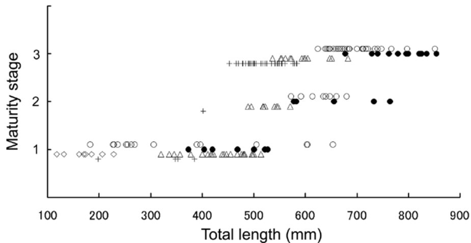
Figure 10. Sexual maturity stages of Apristurus ampliceps sp. nov. (●), A. fedorovi (Δ), A. kampae (+), A. manis (○) and A. stenseni (◇).
