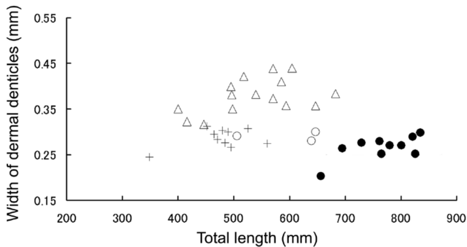
Figure 11. Width of dermal denticles in Apristurus ampliceps sp. nov. (●), A. fedorovi (Δ), A. kampae (+) and A. manis (○).
