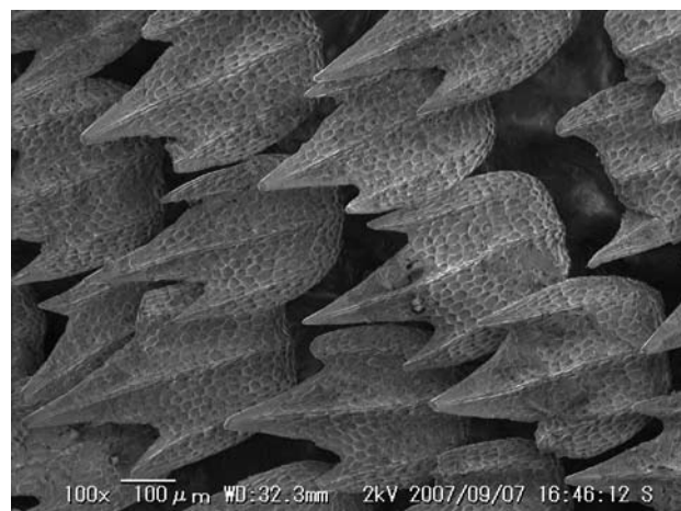
Figure 11. Dermal denticles of Apristurus pinguis : HUMZ 139945, female 546 mm TL. Scale bar = 100 μm.
