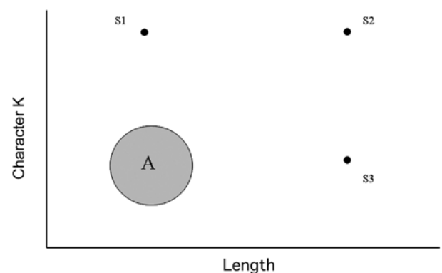
Figure 6. Schematic diagram showing variation and species identification. X-axis, length of the specimen; Y-axis, proportional dimension of character K. Refer to the text for details.
