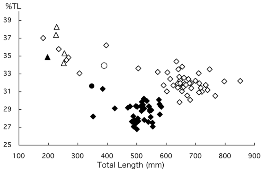
Figure 5. Scatter diagram of proportional dimensions of caudal length in Apristurus kampae and A. manis . Closed symbols, A. kampae ; open symbols, A. manis ; circles, holotypes; triangles, paratypes; diamonds, non-types.
