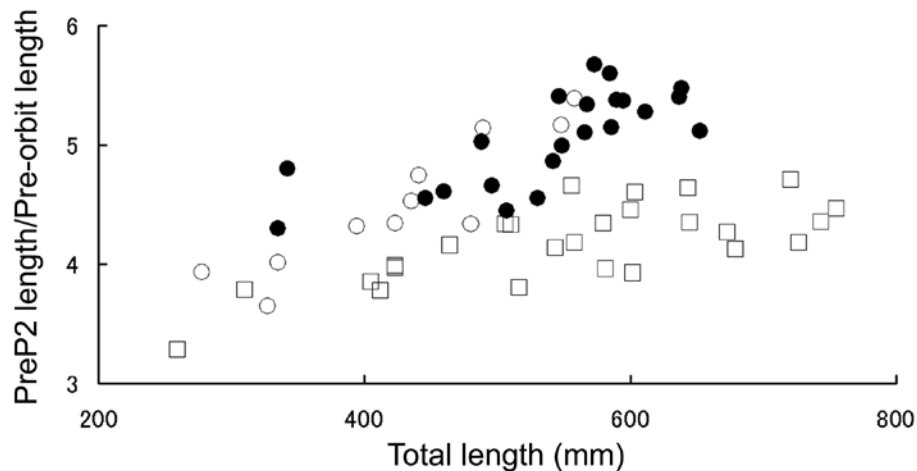
Figure 19. Ratio of pre-orbital length in preP2 length: A. pinguis from the Indian and the western South Pacific (●), from East China Sea (○) and A. profundorum (□).
