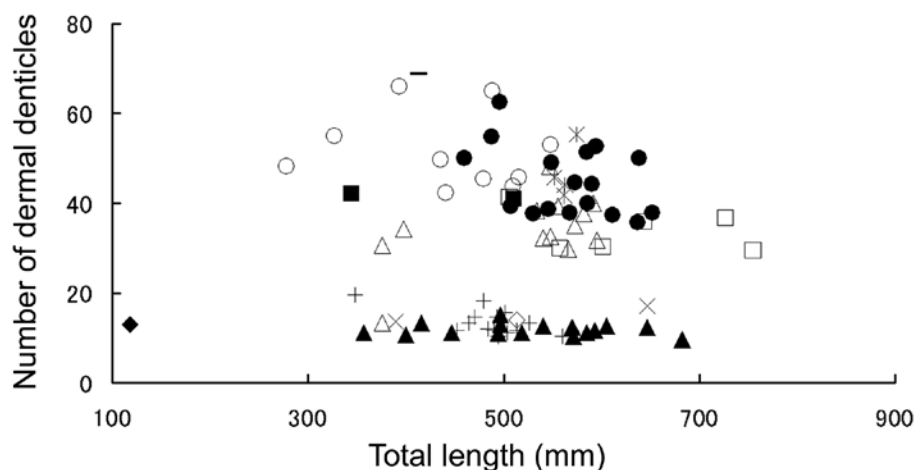
Figure 16. Number of dermal denticles in a 2×2 mm square. A. pinguis from the Indian and the western South Pacific (●) and from the East China Sea (○); A. albisoma (Δ); A. aphyodes (■); A. fedorovi (▲); A. kampae (+); A. manis (×); A. microps (*); A. profundorum (□); A. spongiceps (◇); A. stenseni (◆) and A. riveri (–).
