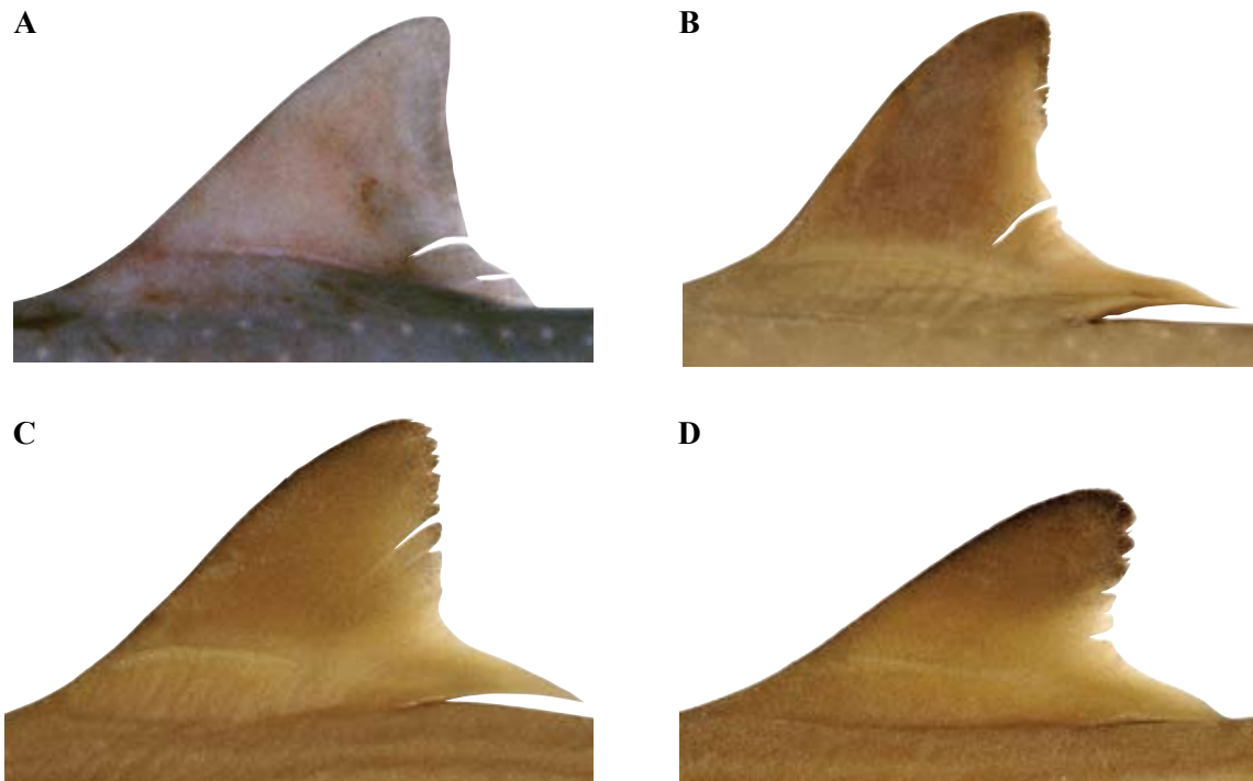
Figure 2. First (A, C) and second (B, D) dorsal fins of Mustelus stevensi sp. nov.: A. (fresh), B. (preserved) holotype, CSIRO H 1035–13 (adult male, 611 mm TL); C., D. juvenile paratype, CSIRO H 4074–15 (male 278 mm TL).
