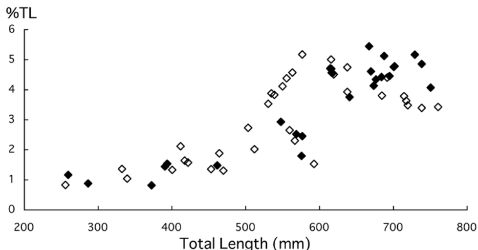
Figure 5. Clasper development in Apristurus melanoasper . ♦, present specimens; ◇, North Atlantic specimens.
