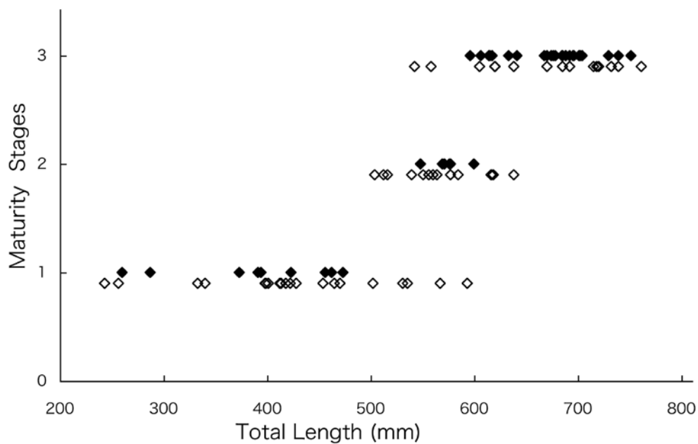
Figure 6. Maturity stages in Apristurus melanoasper . ◆, present specimens; ◇, North Atlantic specimens. 1, immature; 2, adolescent; 3, adult.
