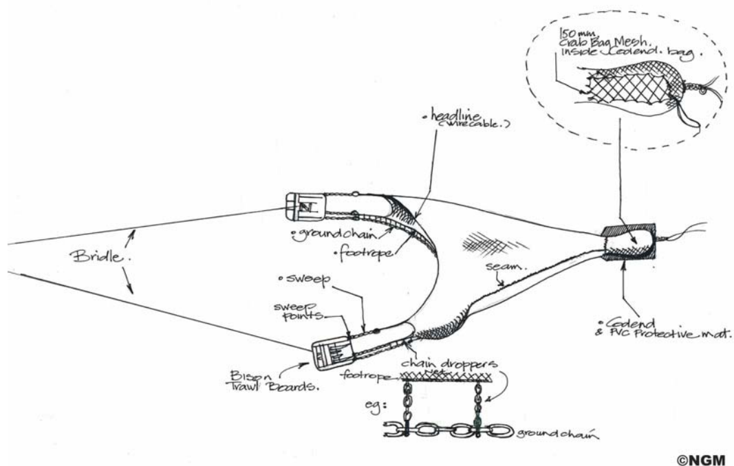
Figure 1.4 Trawl net configuration showing trawl boards, head rope, ground chain and cod end with crab bag. Figure from Carrick (2003).
