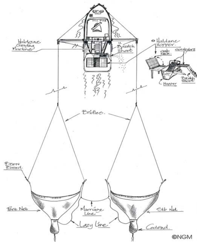
Figure 1.3 Double rig trawl gear and location of hopper sorting and prawn grading systems. Figure from Carrick (2003).
