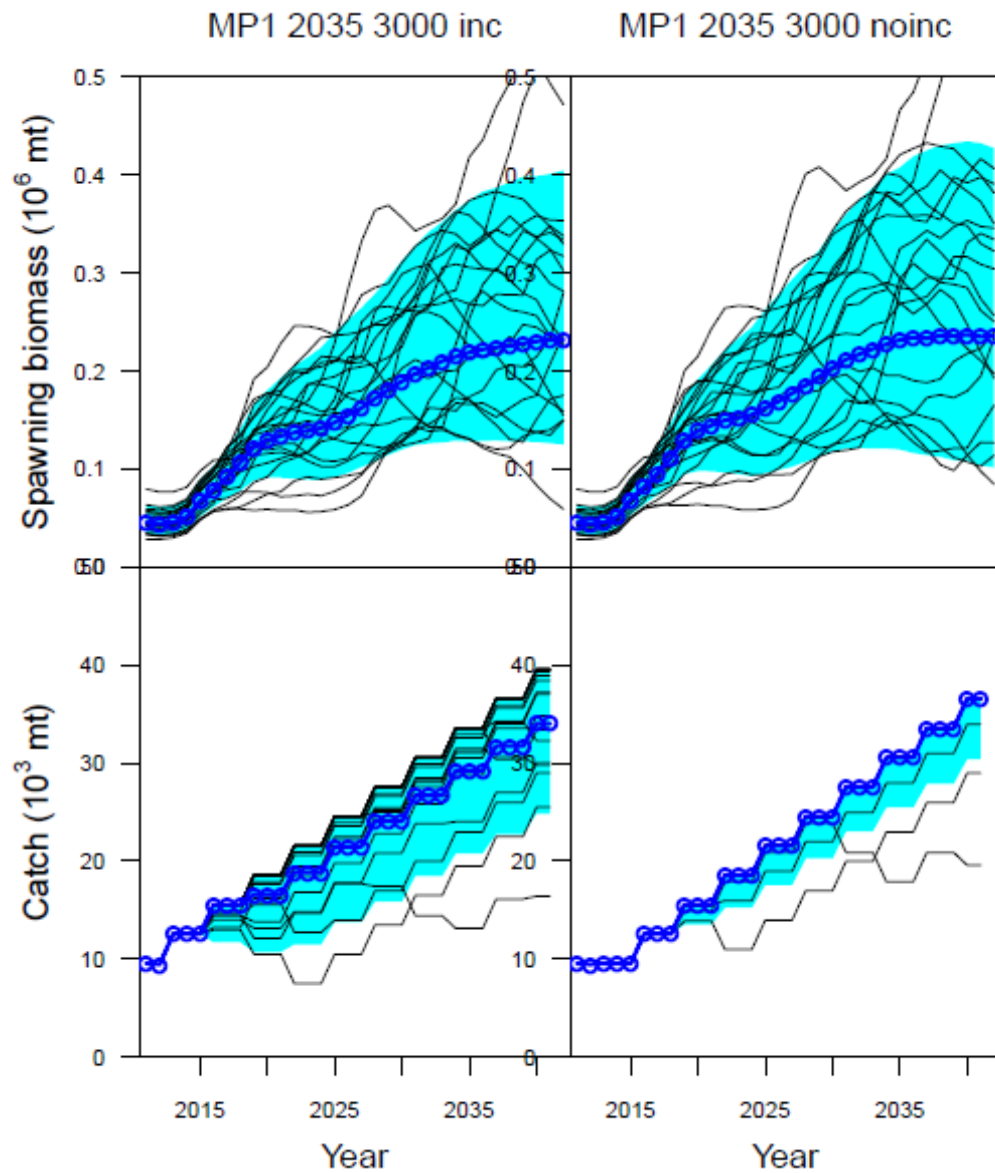
Figure 5. As for Figure 1, except showing only MP1 tuned to meet the objective in 2035 allowing for a 3000 t TAC increase or decrease in any year, comparing the effect of inc and noinc in 2013.
