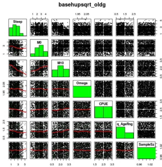
Figure 4a) Sampling of different model parameter values under the old growth schedule.
