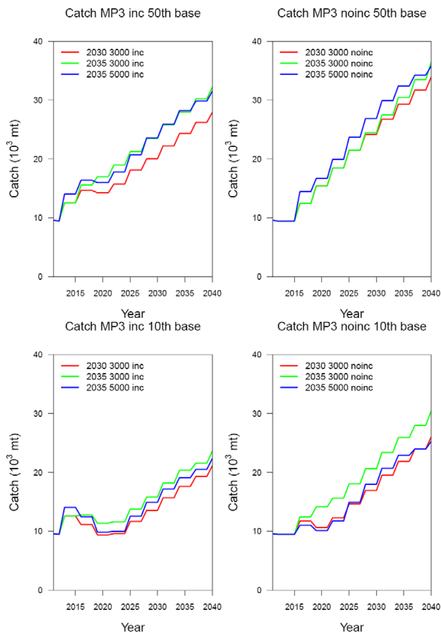
Figure 8. Projected median catch (top row) and 10th percentile of catch (bottom row) for the reference set and a tuning 70% probability of 0.2 SSB_0 by 2030 and 2035 and a maximum TAC change of 3000 and 5000t, with (left column) and without (right column) an increase in TAC in the first implementation year.
