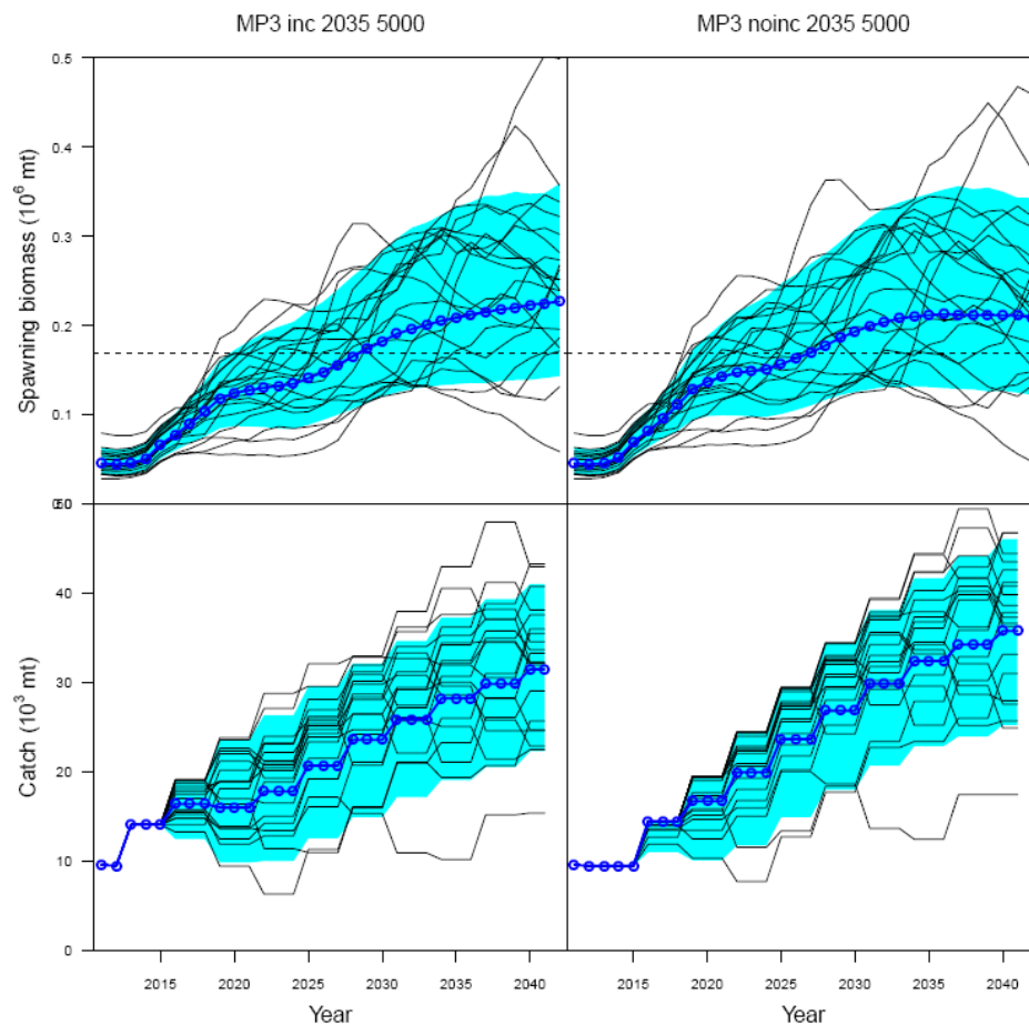
Fig 11a: tuning year 2035 and maximum TAC change of 5000t
